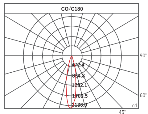
SRL-P20D/7W/3000K/24°
