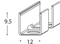
FLEXIBLE ALUMINIUM PROFILE
